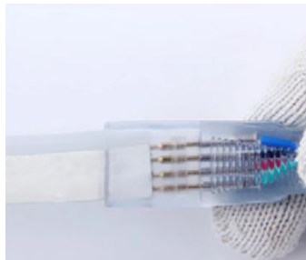
Step 4. Align the 4-Pin connector and insert into the LED RGB controller connector.
